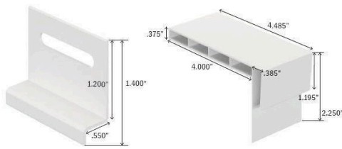
Drip Trim
