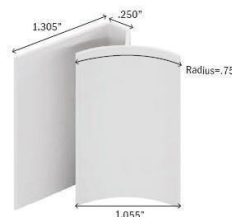
Corner Trim
