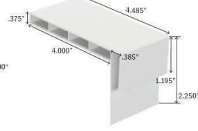
Sill Trim
