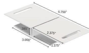
Multi-H Trim
