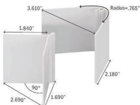
Multi-corner Trim (Male and female)
